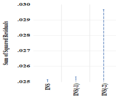
Chart 1: Total Sum of Squared Residuals
